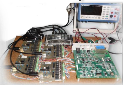
Benchtop Test Fixtures
